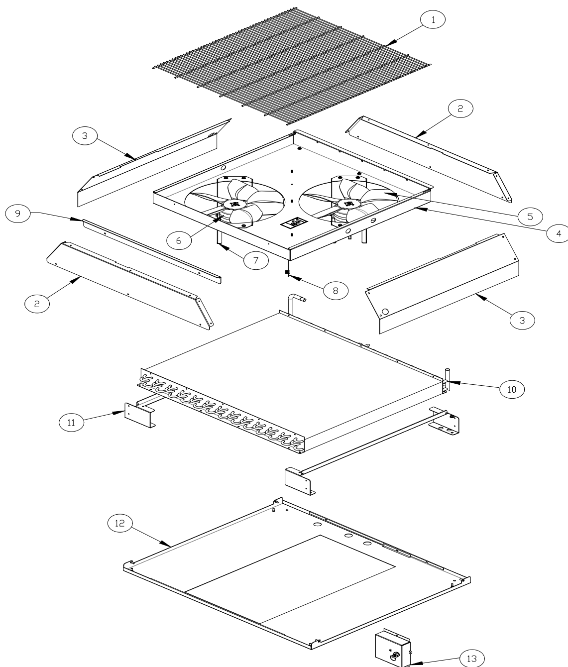
ICE1506 Top Air Discharge
